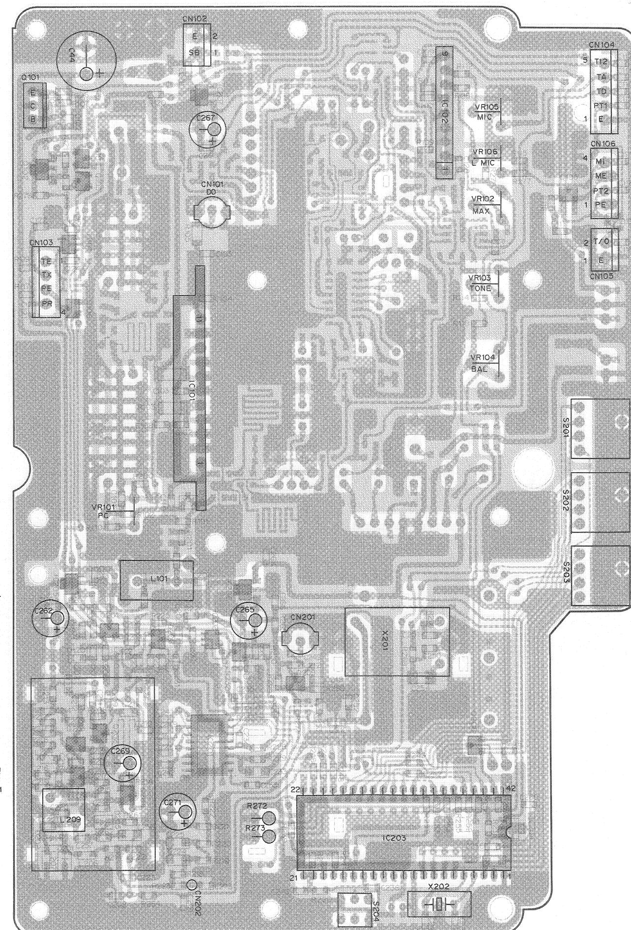
TX UNIT (X56-3020-10) Foil side view
