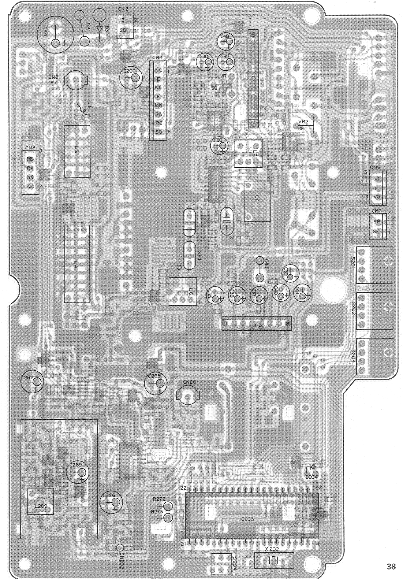
RX UNIT (X55-3020-10) Foil side view
